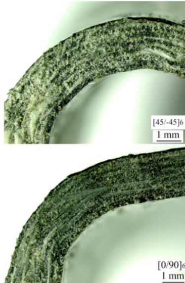
Fig. 2. Optic microscope images of 160°C press formed composite laminates
