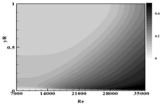
Fig. 2 Distribution of normalized turbulence kinetic energy ( k - \epsilon - \nu^2 results) ( Re = 7000 - 35000 , T=3.8 sec)
