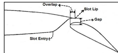
Figure 1. The parameters of airfoil equipped with single slotted flap
