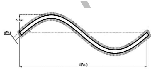
Fig. 2. Specifications of the vortex generators with a sinusoidal wave profile.
